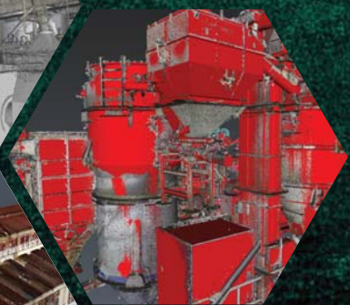
2D and 3D as-is as-built model (Building and Infrastructures)
